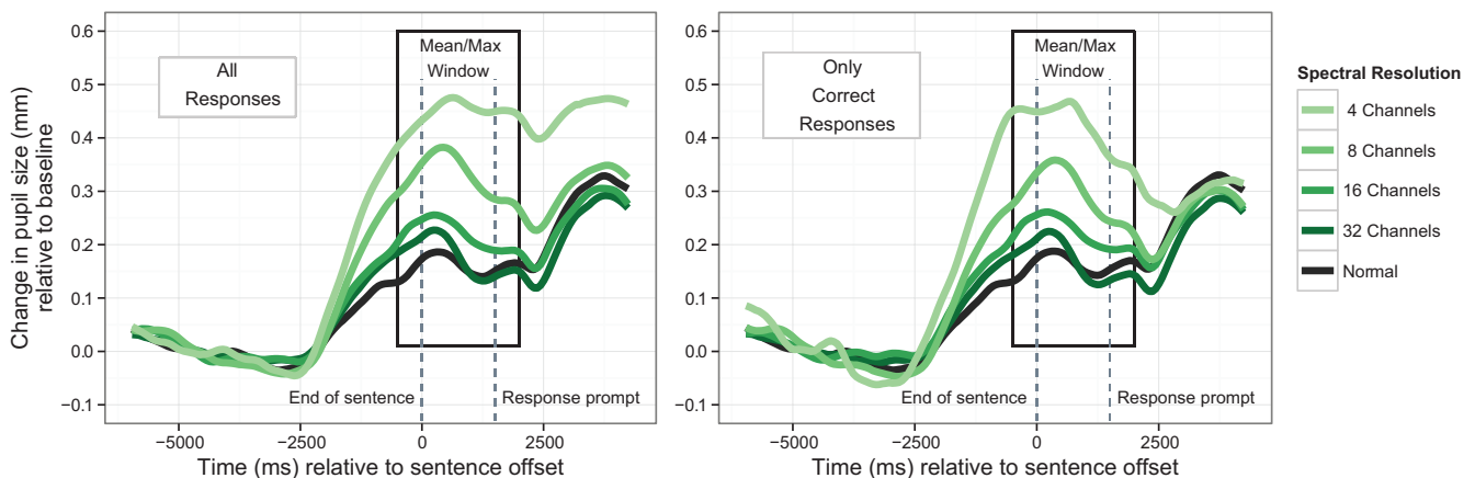
Fig. 1. Change in pupil dilation over time as a function of spectral resolution (number of vocoder channels) in Experiment 1. Time (milliseconds) is plotted relative to stimulus offset. The boxed area represents the time window traditionally used for aggregated analysis. Left panel, data from all trials. Right panel, data only from trials where the entire sentence was identified correctly.
